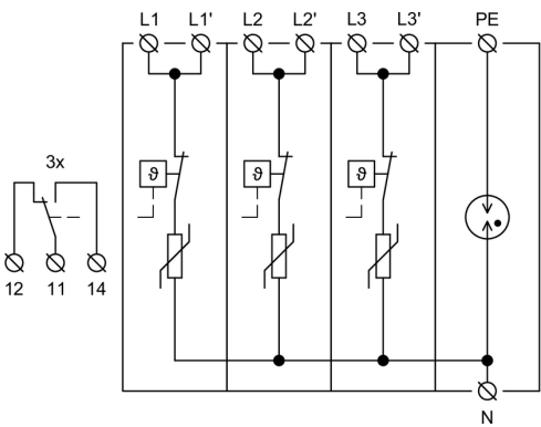
Internal diagram
