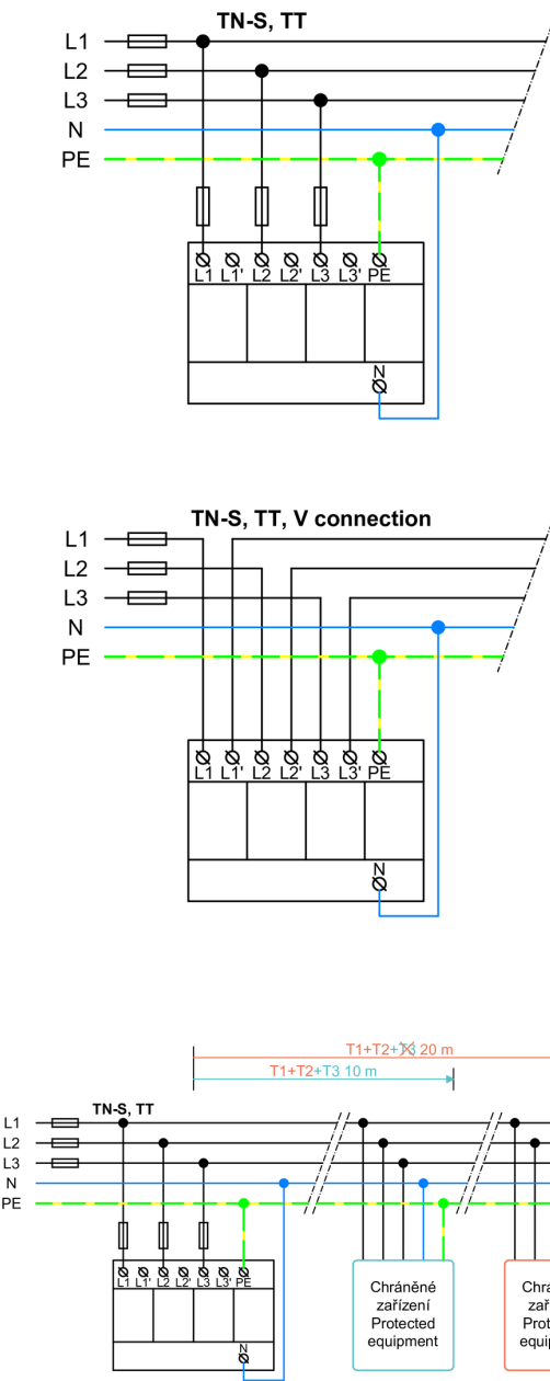
Application wiring diagram (installation)
